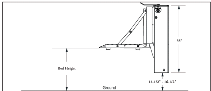
Lift Dimensions
