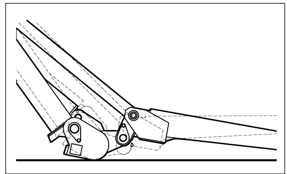
LEVELING JOINT
